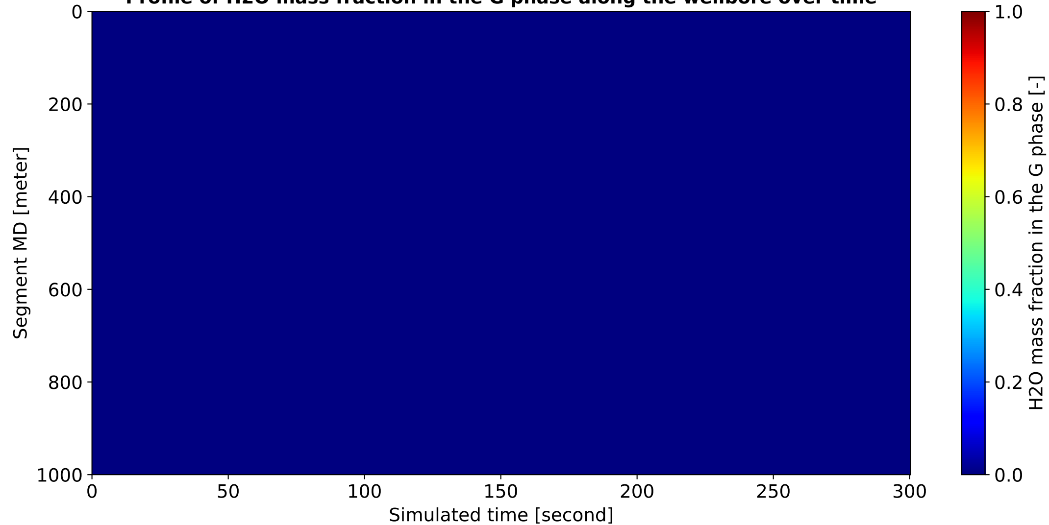
Profile of H2O mass fraction in the G phase along the wellbore over time
